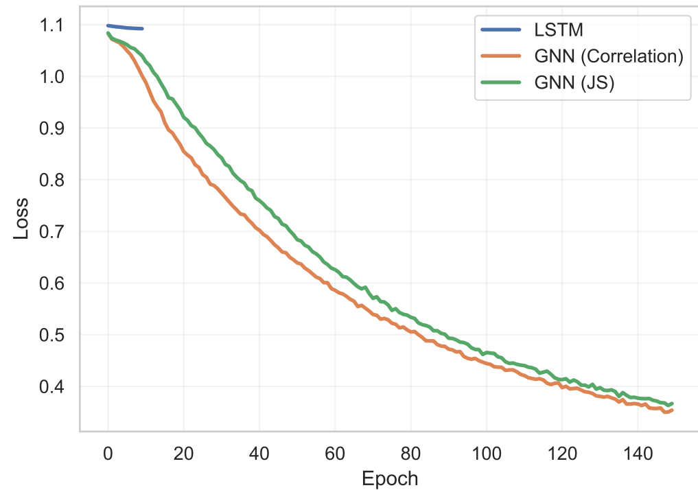
Training loss
